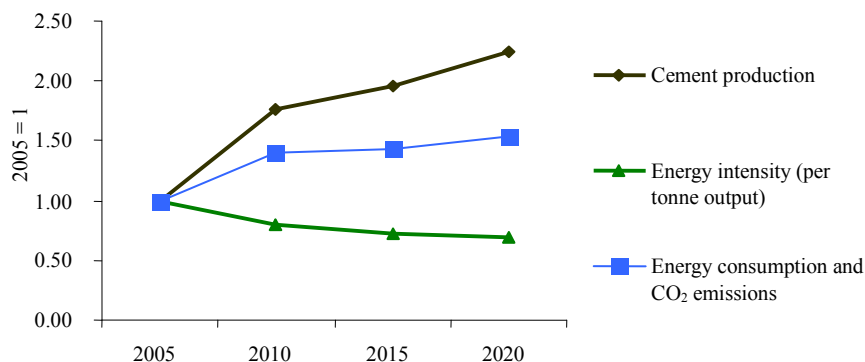
Figure 10 Cement: expected change in production, energy-intensity improvements and total energy consumption by 2020
