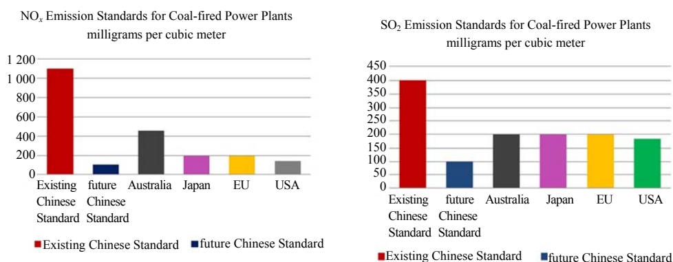
Figure 10 Chinese SO 2 and NO x standards in an international comparison
